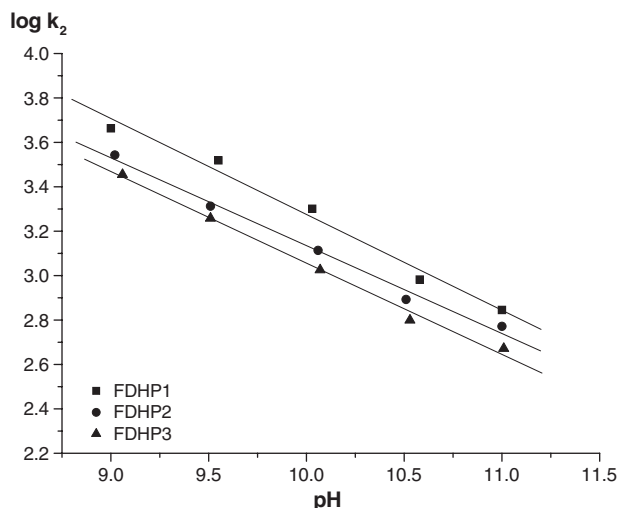
Fig. 4. Disproportionation rate constant dependence on pH for the nitro radical anion of 1 mM nitrofuryl derivatives in mixed medium, 60/40: DMF/citrate buffer (KCl 0.3 M).
