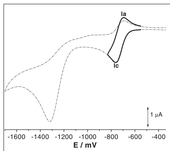
Fig. 2. Cyclic voltammogram of 1 mM FDHP1, in mixed medium at pH 9. Sweep rate 1 V s -1 . Whole line shows a short sweep with the isolated R\text{NO}_2^{\bullet-}/R\text{NO}_2^+ couple.
