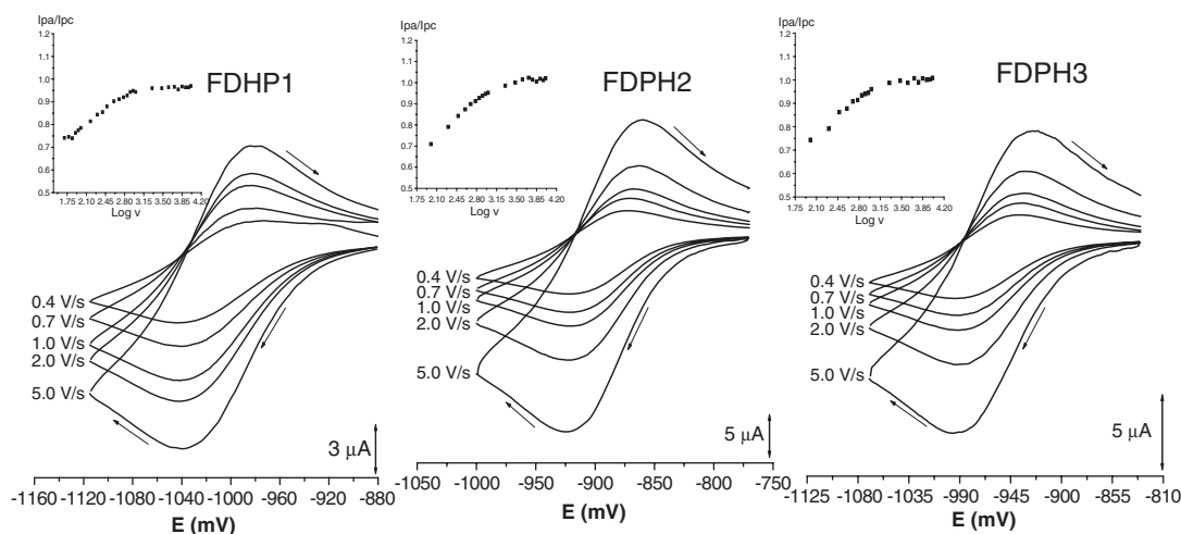
Fig. 5. Cyclic voltammograms of the electrochemically formed \text{R}-\text{NO}_2/\text{R}-\text{NO}_2^{\bullet-} couple from 1 mM solution of FDHP1, FDHP2 and FDHP3 in non-aqueous medium at different sweep rates. Inset: dependence of the current ratio on sweep rate for each set of experiments.
